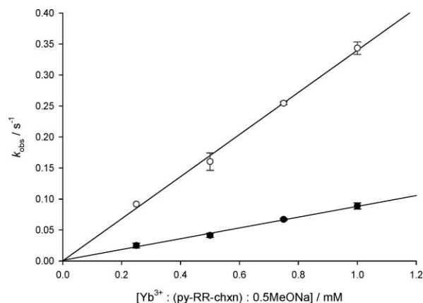
Fig. 1 Plots of k_{\text{obs}} vs. [Pyr-R,R'-chxn:Yb 3+ :0.5(NaOMe)] for methanolysis of D-Boc-Gln-ONp (●) and L-Boc-Gln-ONp (○) (0.05 mmol dm -3 ) in methanol at 25 °C.
