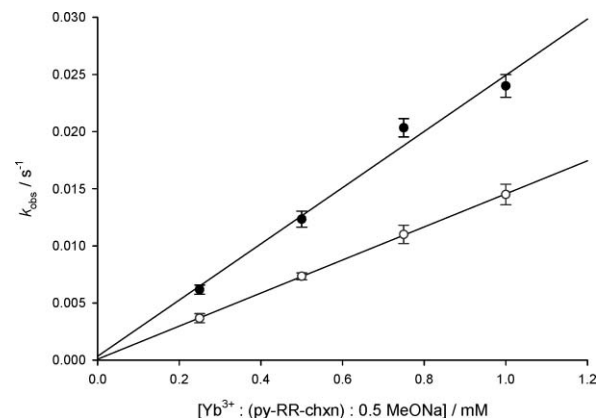
Fig. 2 Plots of k_{\text{obs}} vs. [Pyr-R,R'-chxn:Yb 3+ :0.5(NaOMe)] for methanolysis of D-Boc-Phe-ONp (●) and L-Boc-Phe-ONp (○) (0.05 mmol dm -3 ) in methanol at 25 °C.
