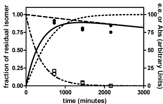
Fig. 5 Time course for various parameters arising from the ethanolysis of D-Boc-Gln-OPNP and (1.0 mmol dm -3 ) and rac-Boc-Gln-OPNP, each promoted by 1.0 mmol dm -3 (Pyr-R,R'-chxn) 2 :La 3+ :(-OEt) in ethanol at -40 °C. Plots are constructed using first order rate constants calculated from activation parameter values ( k^D = 4.53 \times 10^{-5} \text{ s}^{-1} , k^L = 1.12 \times 10^{-6} \text{ s}^{-1} ). Shown are the ee (dotted line, right axis), and the residual fractions of D and L enantiomers vs. time (---, ---, left axis). Solid line is the computed ΔAbs. vs. time plot where the right y-axis represents the maximum absorbance expected for cleavage of one isomer. □ and ● symbols are duplicates of experimentally observed amounts of residual of D and L isomers at times 720, 1440 and 2160 min.
